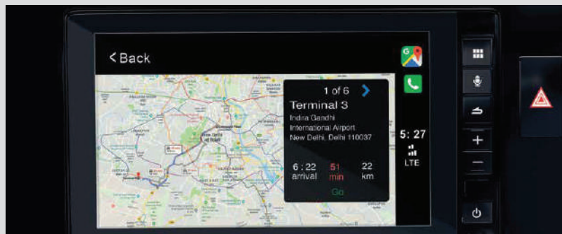
SMARTPHONE NAVIGATION
