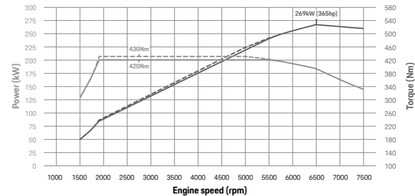
718 Boxster GTS and 718 Cayman GTS: 269kW (365hp) at 6,500rpm — 6-speed manual transmission: 420Nm between 1,900 and 5,500rpm - - - Porsche Doppelkupplung (PDK): 430Nm between 1,900 and 5,000rpm
